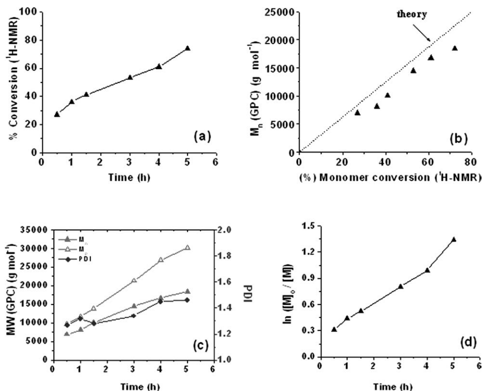
FIGURE 2 Results of the kinetic study of styrene RAFT homopolymerization. (a) Temporal evolution of the conversion of styrene, (b) dependence of M_n on monomer conversion, (c) temporal evolution of the MWs and the PDIs, and (d) pseudo-first-order kinetic plot of the polymerization. [St]_0/[AIBN]_0/[CTA]_0 = 300:0.625:1 , temperature = 110 °C, bulk polymerization.
