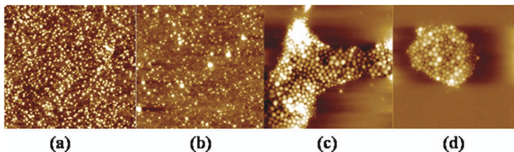
FIGURE 5 Topographic tapping-mode AFM images ( 2\ \mu\text{m} \times 2\ \mu\text{m} scan size) of the reverse micelles formed by the BCs cast from toluene solution ( c = 0.2\ \text{w/v}\% ) (a) \text{St}_{161}\text{-}b\text{-}2\text{VP}_{48} (3 nm), (b) \text{St}_{161}\text{-}b\text{-}2\text{VP}_{121} (3 nm), (c) \text{St}_{161}\text{-}b\text{-}4\text{VP}_{76} (10 nm), and (d) \text{St}_{161}\text{-}b\text{-}4\text{VP}_{107} (17 nm). The values in parentheses indicate the micelle heights measured by AFM.
