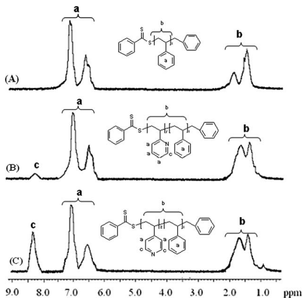
FIGURE 3 1 H NMR spectra of (A) the PSt macroRAFT CTA, (B) St_{161}\text{-}b\text{-}2VP_{48} , and (C) St_{161}\text{-}b\text{-}4VP_{107} , all recorded in CDCl 3 .
