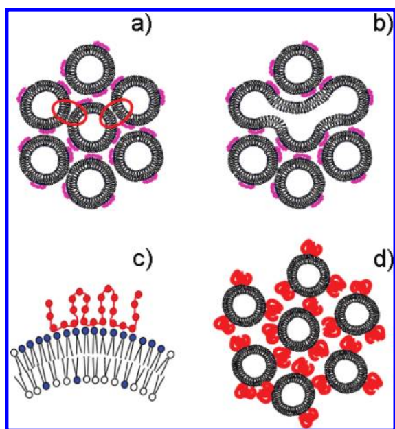
Figure 3. (a, b) Structures of polylysine/liposome complexes (a) before and (b) after fusion. The red ovals in (a) show points of contact between bilayers. (c) Schematic illustration of looping in a PEVP/liposome complex, showing domain formation involving PEVP (red circles) and CL^{2-} (blue circles) embedded in phosphatidylcholine (white circles). (d) Schematic showing how PEVP physically retards the fusion process.
